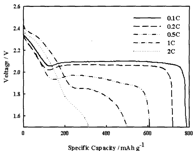
Fig. 3. Discharge rate characteristics comparison at room temperature.
