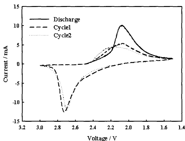
Fig. 2. Cyclic voltammogram of lithium-sulphur battery at a scan rate of 0.1 mV/s.
